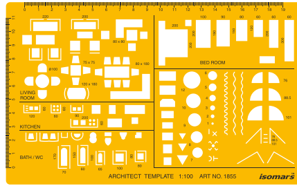
# 1855 - Architect - 1:100 - Size : 219 x 134mm
